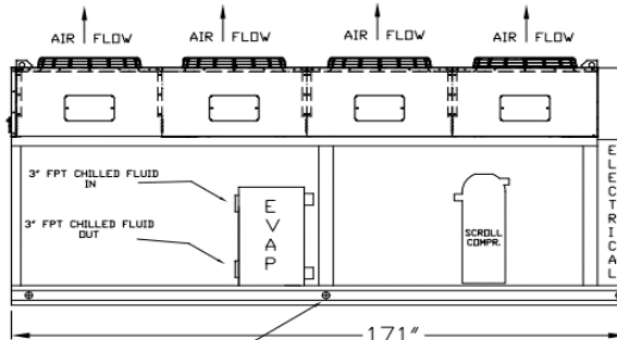
2 1/8" Ø LIFTING HOLES TYP. 8 PLACES LEFT PROFILE
